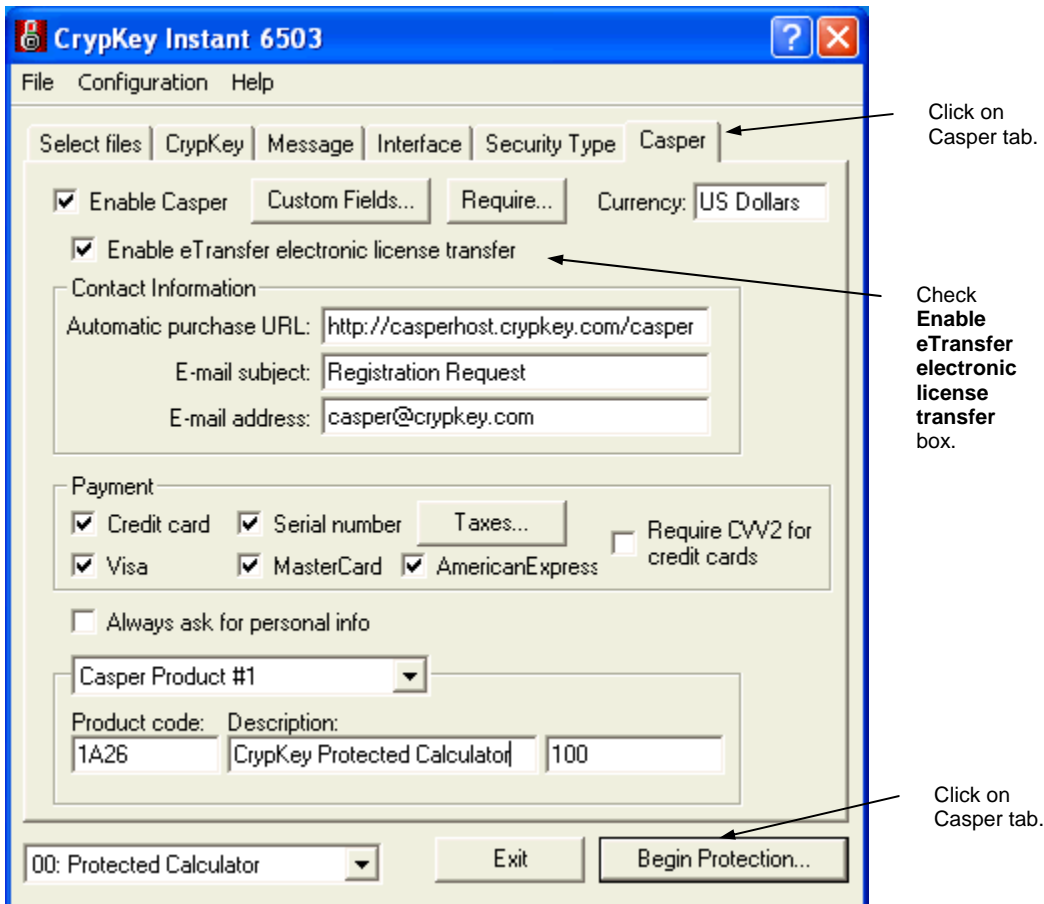
Figure 2-1 Enable eTransfer tab – CrypKey Instant
